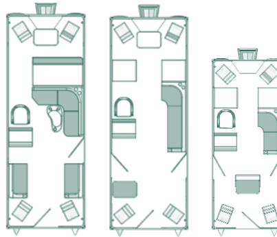
2486-D DLX 7,31-2,59-D DLX 2486-F DLX 7,31-2,59-F DLX 2080-F DLX 6,48-2,44-F DLX pieds mètres
